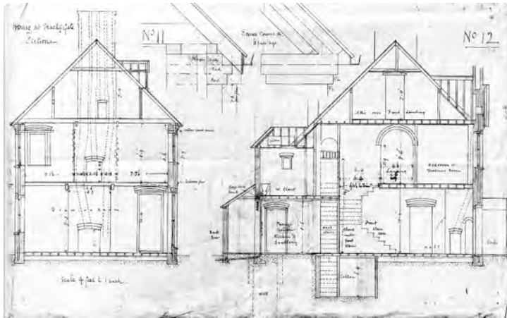
88 Thomas Hardy. Sectional drawings for Max Gate. 'House at Mack's Gate, Sections. No. 11 and No. 12.' Reproduction of the original drawing courtesy of the Dorset County Museum.
